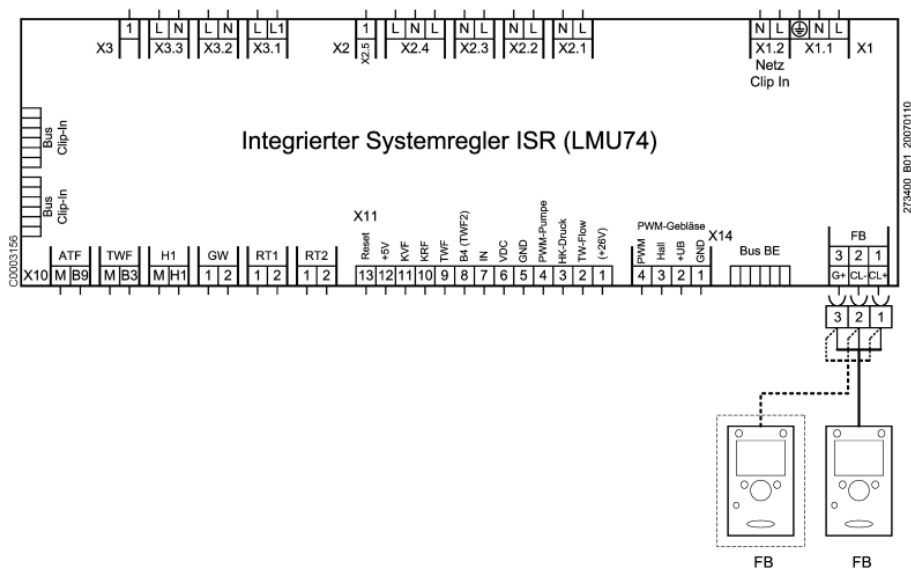
Fig. 3: Wiring diagram for connection to ISR-LMU system controller (from LMU 74)
