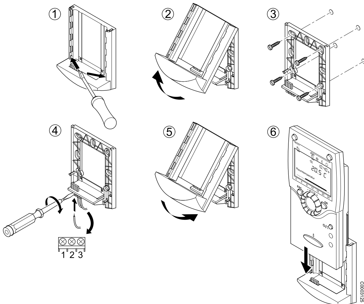
Fig. 6: Installation of the RGT/RGTK room controller
