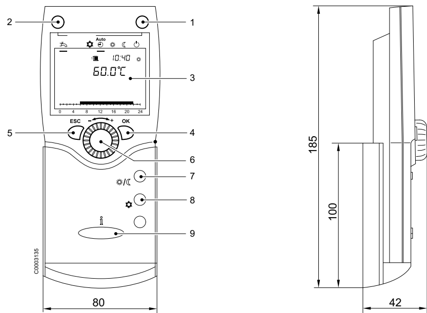
Fig. 1: Overview and dimensions
